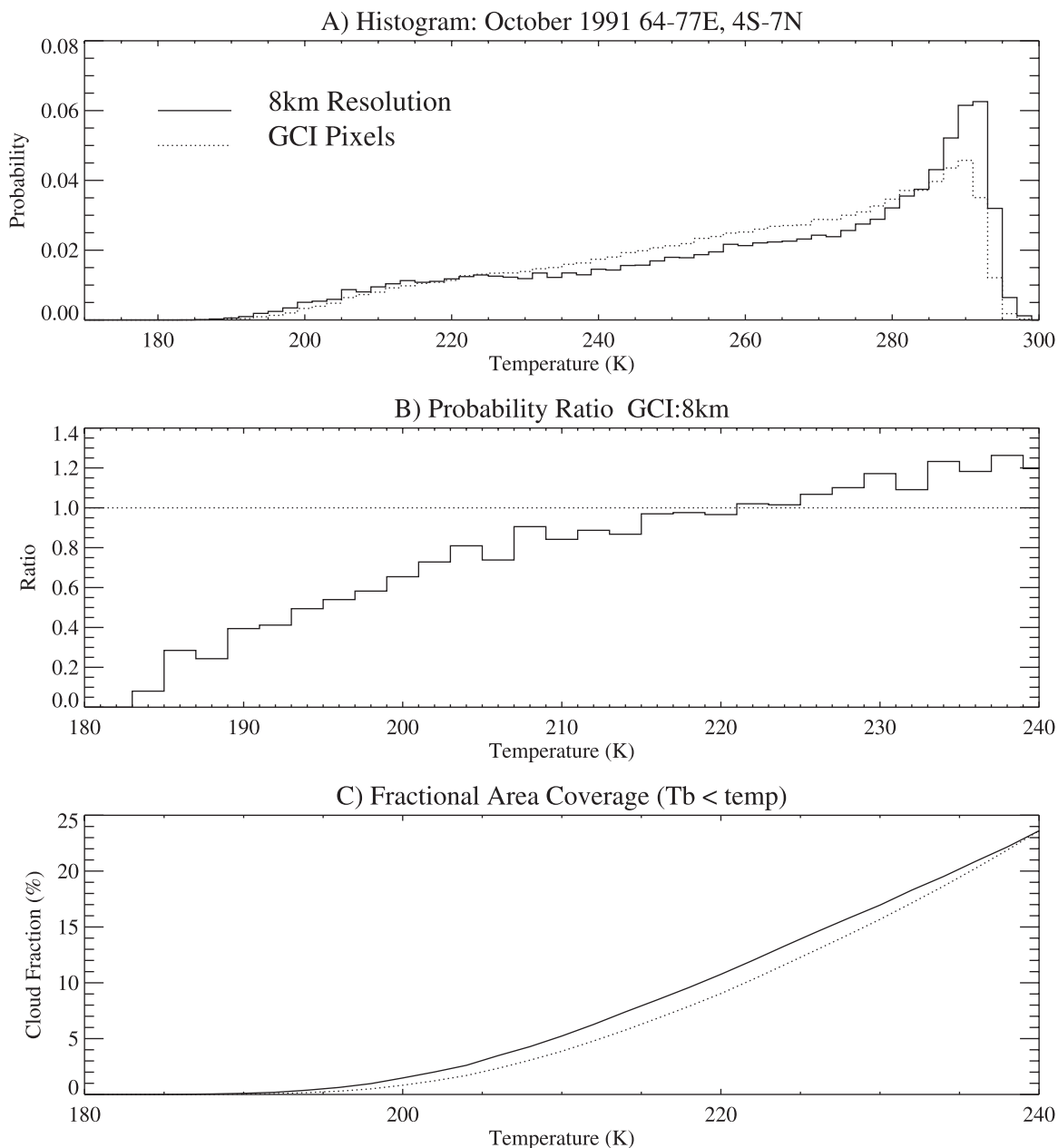
Figure 2. (a) Normalized histogram of brightness temperatures for October 1991 in the region from 64°–77°E and 4°S–7°N. (b) Ratio of GCI probability to 8-km probability in Figure 2a for the coldest temperatures (note different temperature scale from Figure 2a). Dotted line is 1:1 line. (c) Cumulative distribution of cloud fraction colder than a given temperature threshold for the same region as Figure 2a. In Figures 2a and 2c the solid line is from the 8-km data, and the dotted line is from the GCI pixels.
