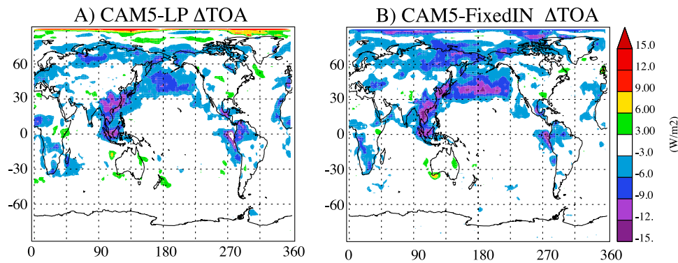
Figure 6. AIE from ice clouds estimated by change in Top of Atmosphere (TOA) radiation ( dR ) between 2000 and 1850 from (a) CAM5-LP and (b) CAM5-FixedIN simulations.
