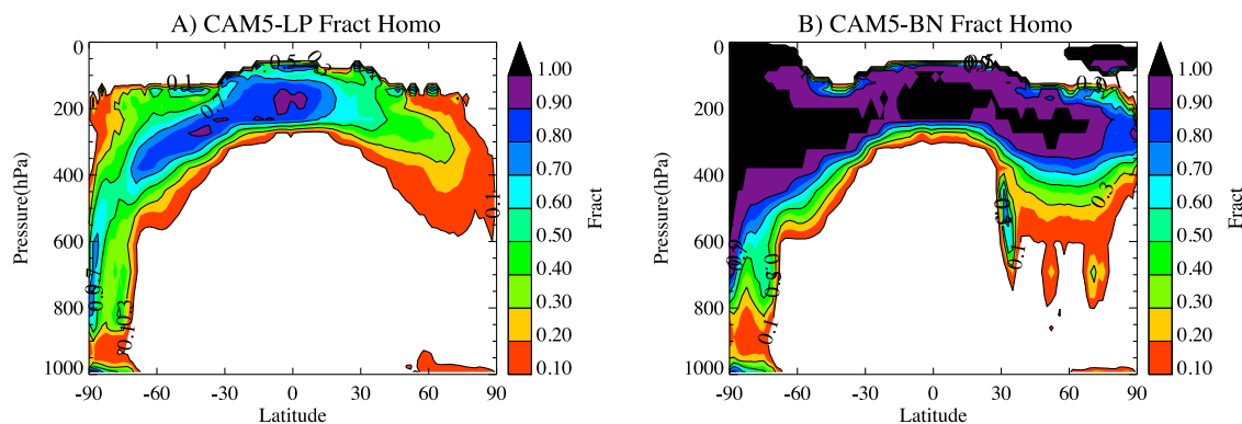
Figure 4. Zonal Mean fraction of activated IN due to homogeneous nucleation in the year 2000 (a) CAM5-LP and (b) CAM5-BN simulations.
