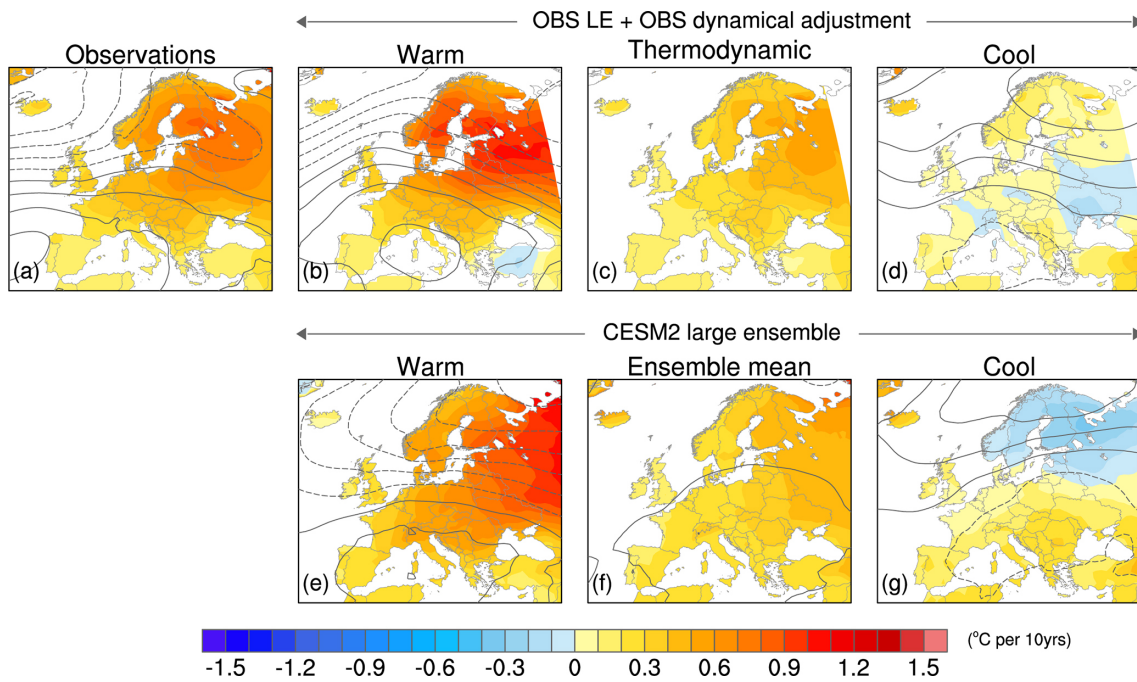
Figure 14. As in Fig. 10 but for the period 1962–2021. The top row (a–d) is based on the observational large ensemble combined with the residual thermodynamic component of observed trends. The bottom row (e–g) is based on the 100-member CESM2 large ensemble. See text for details.
