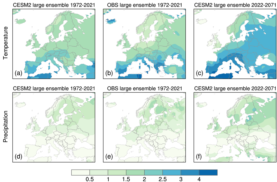
Figure 8. Signal-to-noise ratio of forced trends in winter (a–c) air temperature and (d–f) precipitation based on the 100-member CESM2 large ensemble during 1972–2021 (a, d), the observational large ensemble during 1972–2021 (b, e), and the CESM2 large ensemble during 2022–2071 (c, f). See text for details.
