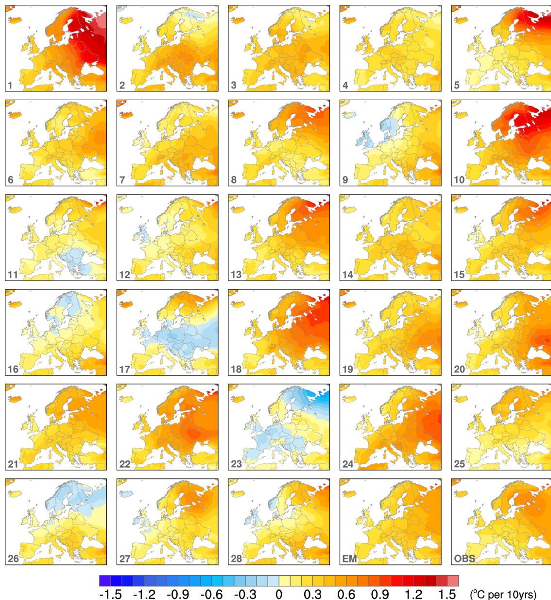
Figure 1. Winter air temperature trends ( ^{\circ}\text{C} per decade) for the period 1972–2021, as simulated by the first 28 members of the CESM2 large ensemble (number in the lower left of each panel denotes the ensemble member) and the 100-member ensemble mean (panel labeled EM). Observed trends are shown in the lower right (panel labeled OBS).
