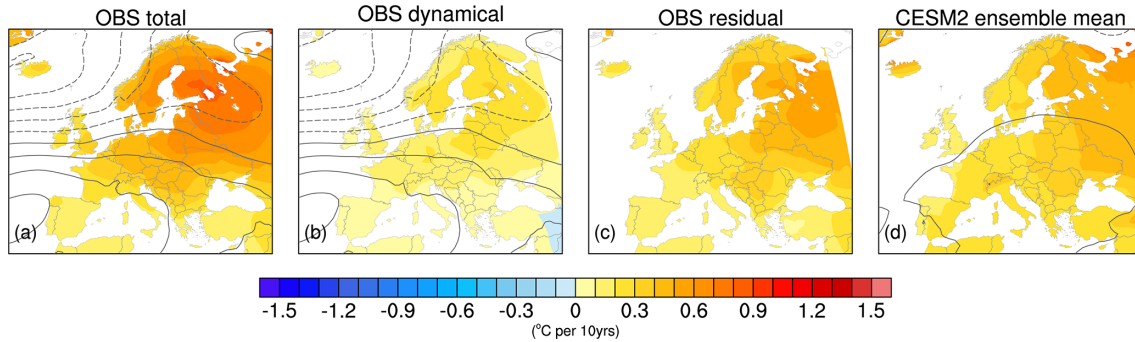
Figure 12. Decomposition of (a) observed winter air temperature trends (1962–2021; °C per decade) into (b) dynamical and (c) residual thermodynamic contributions, using the dynamical adjustment procedure of Deser et al. (2018), based on constructed circulation analogues (see text for details). Contours in panel (a) show observed sea level pressure (SLP) trends (contour interval of 0.25 hPa per decade; negative values dashed), contours in panel (b) show the observed SLP trends estimated from the constructed circulation analogues, and contours in panel (c), based on the difference between panels (a) and (b), are near zero and not shown. Panel (d) shows the ensemble-mean temperature and SLP trends from the 100-member CESM2 large ensemble (note that only the zero contour shows up in panel d).
