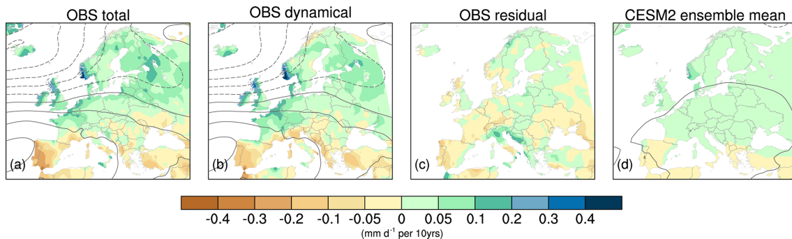
Figure 13. As in Fig. 12 but for precipitation ( \text{mm d}^{-1} per decade).
