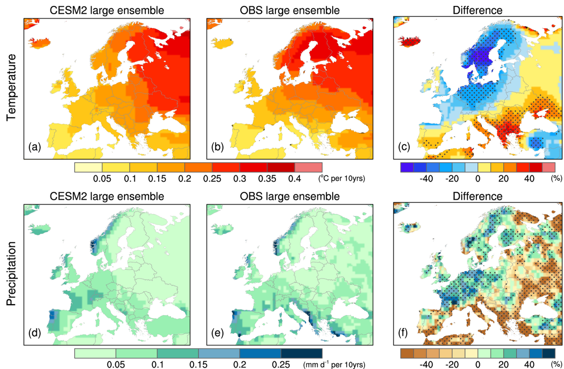
Figure 7. Standard deviation of 50-year trends (1972–2021) across 100 members of the CESM2 large ensemble (a, d) and 100 members of the observational large ensemble (b, e), and their difference (c, f) for winter air temperature (a–c; °C per decade) and precipitation (d–f; mm d -1 per decade). Stippling in panels (c) and (f) indicates that the differences are statistically significant at the 95 % confidence level according to an f test.
