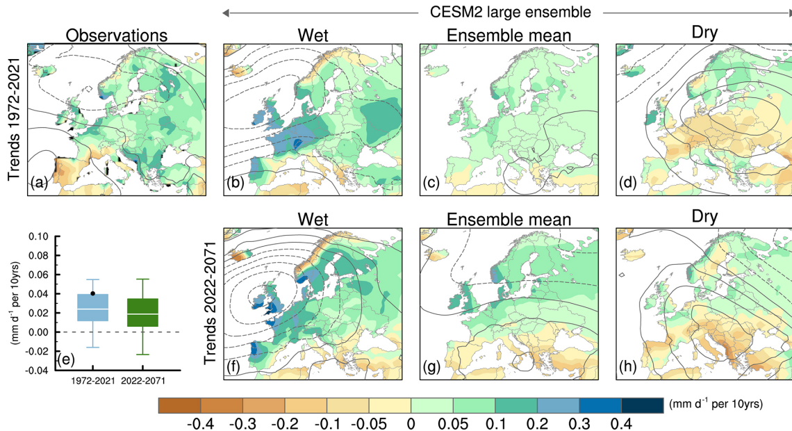
Figure 11. As in Fig. 10 but for precipitation ( \text{mm d}^{-1} per decade). Note that panels (a) and (c) are identical to the OBS and EM panels in Fig. 2, respectively.
