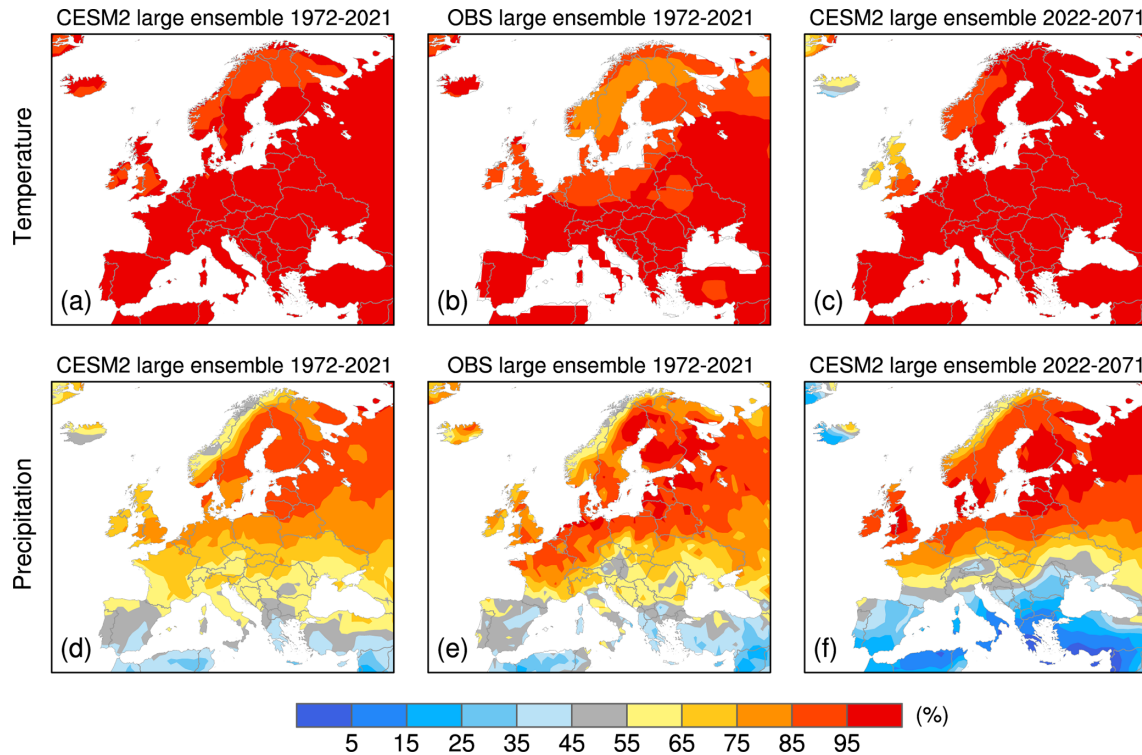
Figure 9. The percentage of ensemble members with a positive trend in winter (a–c) air temperature and (d–f) precipitation trends based on (a, d) the 100-member CESM2 large ensemble during 1972–2021, (b, e) the 100-member observational large ensemble during 1972–2021, and (c, f) the 100-member CESM2 large ensemble during 2022–2071.
