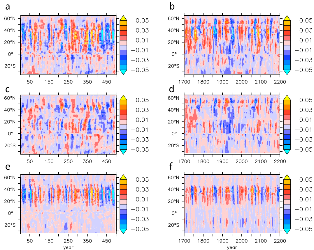
FIG. 6. Modeled Fov(y) anomalies ( Sv ) as a function of time and latitude in (a) ESM2M and (b) CESM1, and their contributions from (c),(d) salinity and (e),(f) velocity anomalies, respectively. Shown are 7-point running averages of the original annual time series with no meridional smoothing applied.
