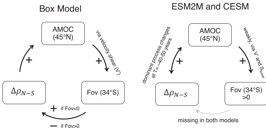
FIG. 12. Physical links underlying the basin-scale salt-advection feedback as envisioned by box models and their counterparts in ESM simulations. In both panels, rectangles represent (clockwise from the top) AMOC at 45°N (used as an AMOC index), Fov(y) at 34°S, and NA–SA density difference ( \Delta\rho_{N-S} ), respectively. Arrows represent forcing from one variable to the next, with the + or – signs indicating if the forcing effect is positive or negative. Based on (left) box models, stronger AMOC at 45°N increases Fov by changing the velocity shear at 34°S, and therefore the arrow connecting them is marked as positive. The forcing from Fov to \Delta\rho_{N-S} can be either positive or negative depending on the sign of Fov: when Fov < 0, stronger Fov increases \Delta\rho_{N-S} (because more freshwater is transferred out of the Atlantic Ocean), and therefore the arrow is positive; when Fov > 0, stronger Fov decreases \Delta\rho_{N-S} (because more freshwater is transferred into the Atlantic Ocean), and the arrow is therefore negative; last, stronger \Delta\rho_{N-S} strengthens AMOC, another positive link. Together, these links form a closed feedback loop; in particular, a negative Fov allows for continuous positive effect to propagate around the loop, destabilizing AMOC, whereas a positive Fov breaks the continuous positive forcing around the loop, stabilizing AMOC. (right) This conceptual model is revised based on analyses on internal variability of AMOC in full ESM simulations where it is found that 1) AMOC45N influences Fov only weakly through either the velocity shear or lower-layer salinity distributions; 2) effect from Fov on \Delta\rho_{N-S} is not detected in both ESMs; and 3) the relationship between AMOC45N and \Delta\rho_{N-S} (the latter is almost entirely controlled by subpolar NA density variations with negligible contributions from SA) is time scale- and process-dependent: on decadal and multidecadal time scales ( T < 40\text{--}50 yr), AMOC variability lags the thermal effect-dominated density variation in both models; on longer time scales ( T > 40\text{--}50 yr), density variation is dominated by the haline effect, and AMOC variability lags density variation in ESM2M but leads it in CESM1 (hence, we draw a double pointed arrow between AMOC45N and \Delta\rho_{N-S} ).
