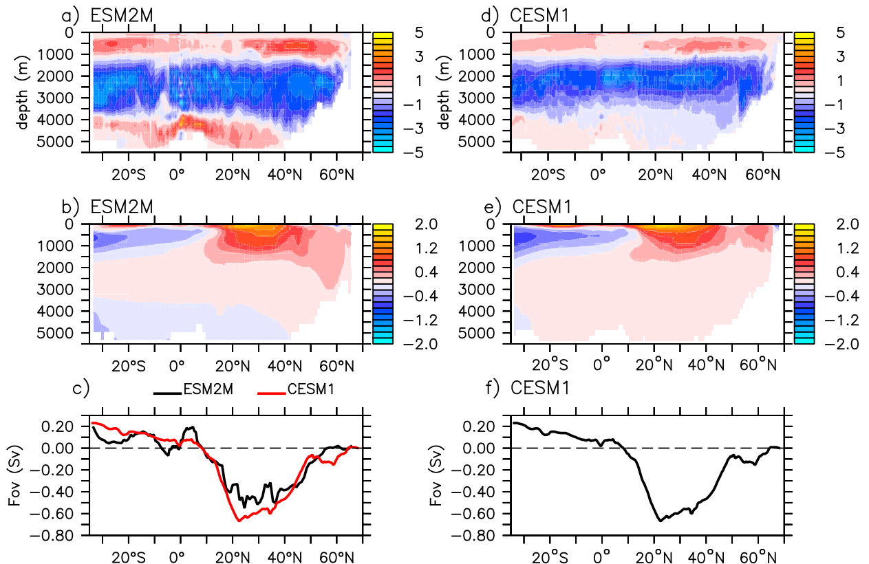
FIG. 1. Long-term mean Atlantic Ocean zonally integrated baroclinic meridional velocity [ \text{Sv} ( 1 \text{ Sv} \equiv 10^6 \text{ m}^3 \text{ s}^{-1} )] in (a) ESM2M and (d) CESM1. Zonally averaged salinity minus 35 (psu) in (b) ESM2M and (e) CESM1. Freshwater transport by AMOC at each latitude, Fov(y) (Sv), in (c) ESM2M and (f) CESM1. The CESM1 result is redrawn in (c) (red line). No meridional smoothing is applied.
