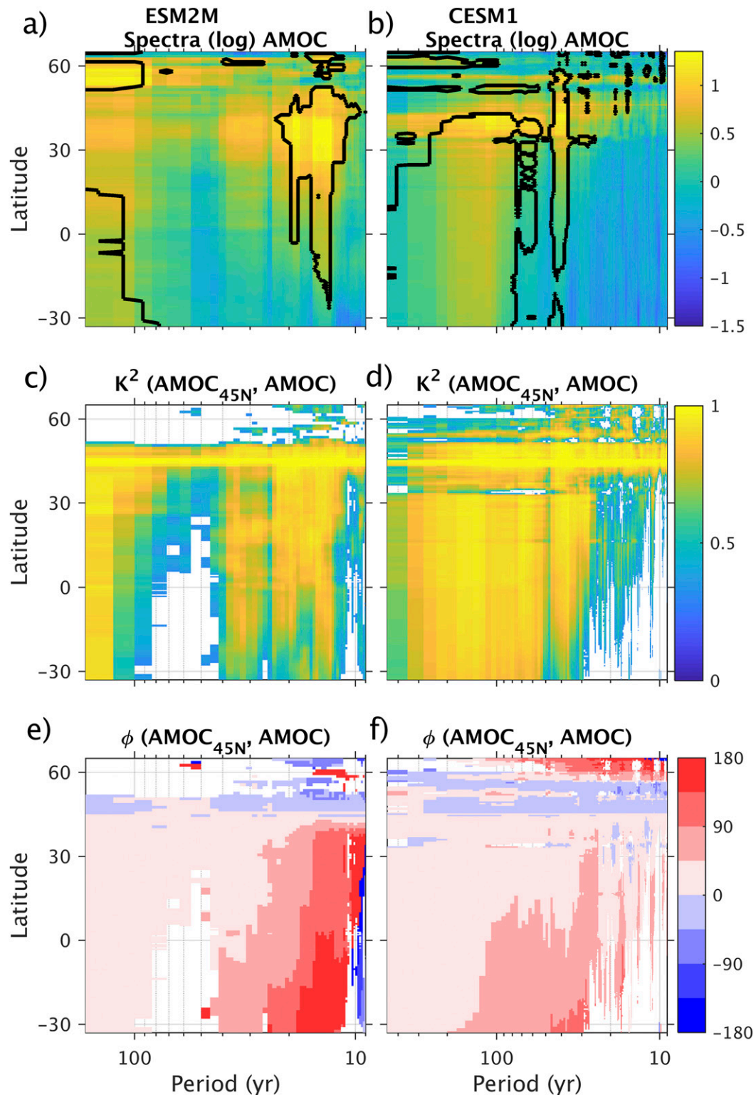
FIG. 9. Spectral analysis of AMOC in (left) ESM2M and (right) CESM1 vs latitude. (a),(b) Logarithm of spectral energy of AMOC(y). Black contours indicate where the spectra differ from a red-noise process with 90% confidence. (c),(d) Squared coherence and (e),(f) coherence phase between AMOC 45N and AMOC(y). Positive (negative) phase means AMOC 45N leads (lags) AMOC(y). Values are only plotted where coherence is significant at 90%. Significance is tested against the 90th percentile of 1000 synthetic time series with the same first-order autoregressive (AR-1) characteristics as the best fit to the original time series. Spectral estimates are filtered with a 7-point Daniell filter (von Storch and Zwiers 1999).
