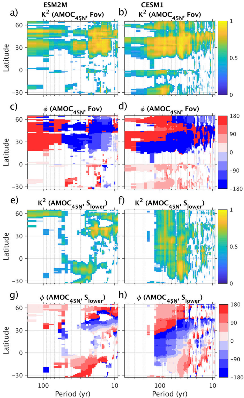
FIG. 10. Squared coherence and coherence phase between AMOC 45N and (a)–(d) Fov(y) and (e)–(h) lower-layer salinity (salinity averaged zonally across the Atlantic, and between 1 and 3 km depth). Positive (negative) phase means AMOC 45N leads (lags) the field. Values are only plotted where coherence is significant at 90%. Significance is tested against the 90th percentile of 1000 synthetic time series with the same AR-1 characteristics as the best fit to the original time series. Spectral estimates are filtered with a 7-point Daniell filter (von Storch and Zwiers 1999).
