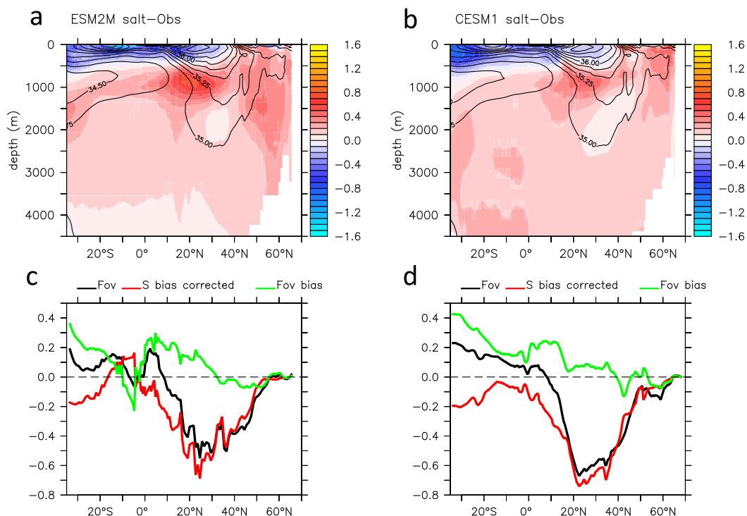
FIG. 2. Long-term mean Atlantic zonally averaged salinity bias (model – observation; psu; color shading) and observed zonally averaged salinity (psu; black contours) in (a) ESM2M and (b) CESM1. Long-term mean Fov(y) (black line), resulting Fov(y) when salinity bias is removed in computing Fov(y) (red line), and difference between original and salinity bias–corrected Fov(y) (green line) in (c) ESM2M and (d) CESM1. Units in (c) and (d): Sv.
