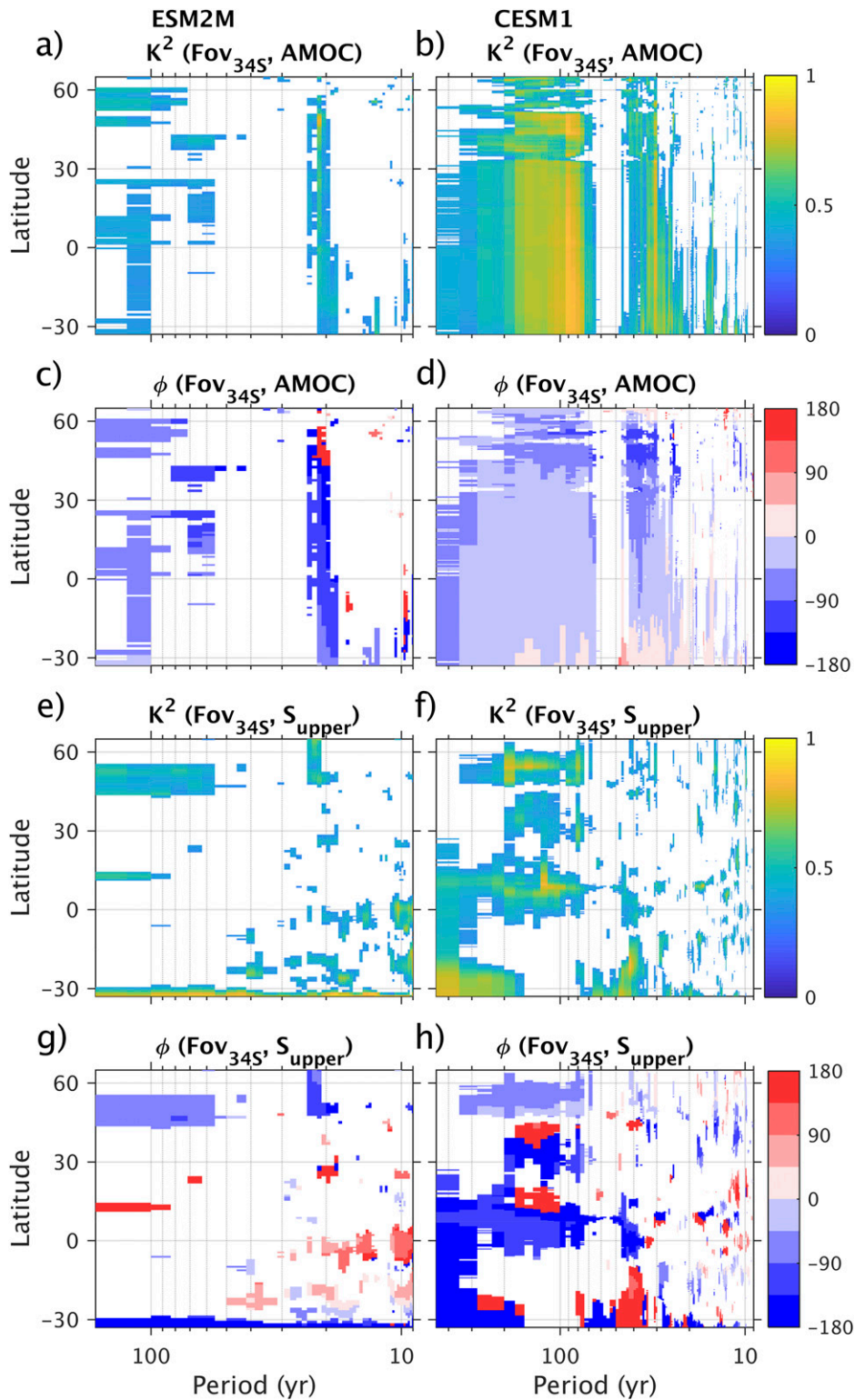
FIG. 11. As in Fig. 10, but for the coherence between Fov and (a)–(d) AMOC(y) and (e)–(h) upper-layer salinity (salinity averaged zonally across the Atlantic, and between 100 m and 1 km depth). Positive (negative) phase means Fov leads (lags) the field.
