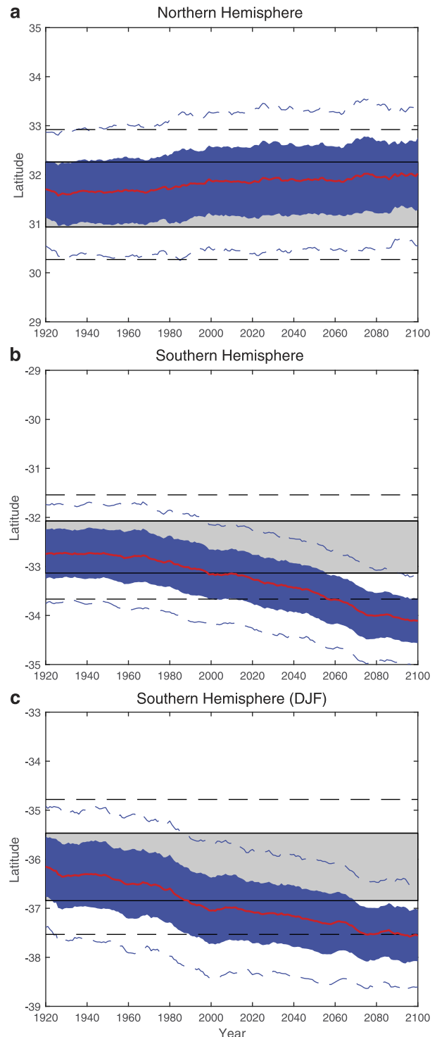
FIG. 5. Latitudes of (a) NH annual-mean tropical edge, (b) SH annual-mean tropical edge, and (c) SH DJF-mean tropical edge over the 1920–2100 period from the CESM-LE, as measured by the USFC metric. The 40-member ensemble mean (smoothed with a 10-yr running mean) is in red, with the one- and two-standard-deviation ranges across ensemble members marked with blue shading and blue dashed lines, respectively. The one- and two-standard-deviation ranges in the control run of the model are marked with gray shading and black dashed lines, respectively.
