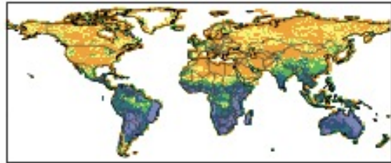
cam6clm50sp_cesm23a02cPPEn08ctsm51d030_1deg_hist DJF
