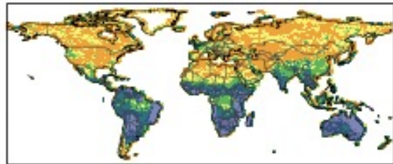
cam6ctsm51sp_cesm23a02cPPEn08ctsm51d030_1deg_hist
