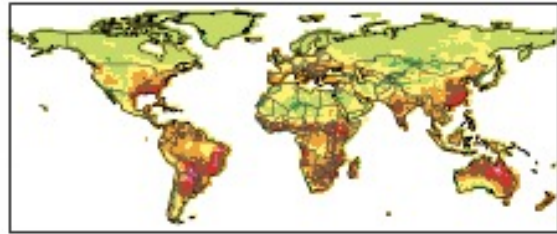
cam6clm50sp_cesm23a02cPPEn08ctsm51d030_1deg_hist DJF
