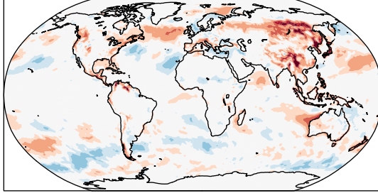
SON PBLH Daily 00
