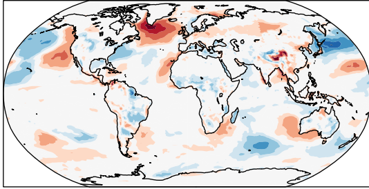
JJA PBLH Daily Mean
