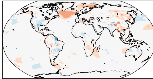
ANN PBLH Daily Mean
