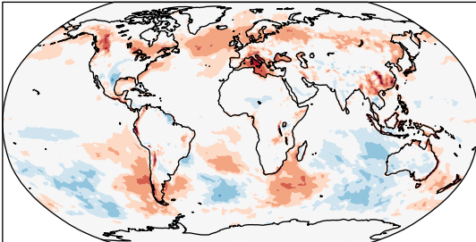
ANN PBLH Daily 00
