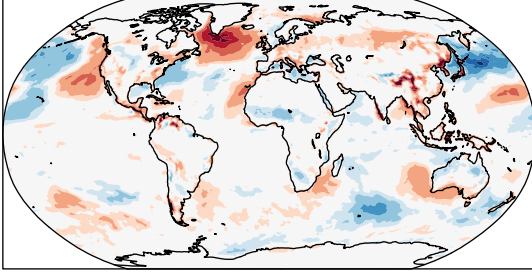
JJA PBLH Daily 00
