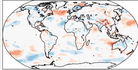
SON PBLH Daily Mean
