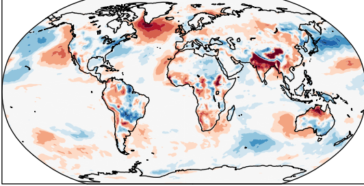
JJA PBLH Daily 12
