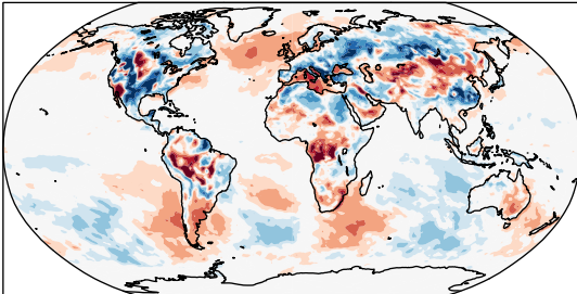
ANN PBLH Daily 12
