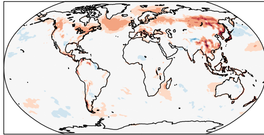
ANN PBLH Daily 00
