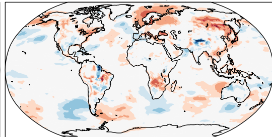
ANN PBLH Daily Mean
