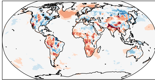
ANN PBLH Daily 12
